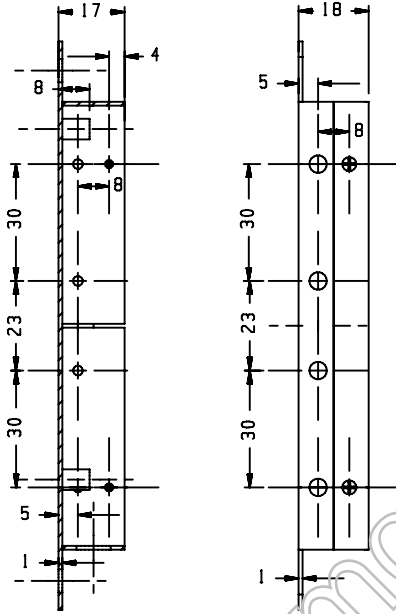
SECTION J - J
