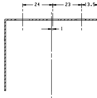
SECTION J - J
